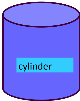
mathematics
