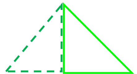
symmetry
